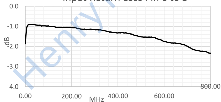
Input Return Loss Pin 6 to 3
