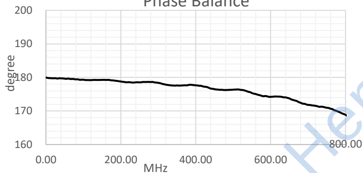
Phase Balance
