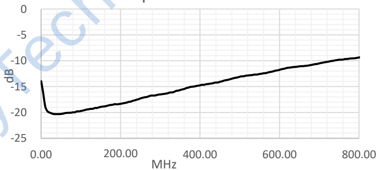
Input Return Loss
